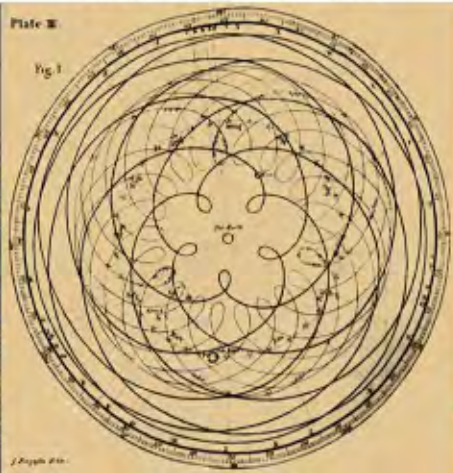
Orbital Pattern of Venus
